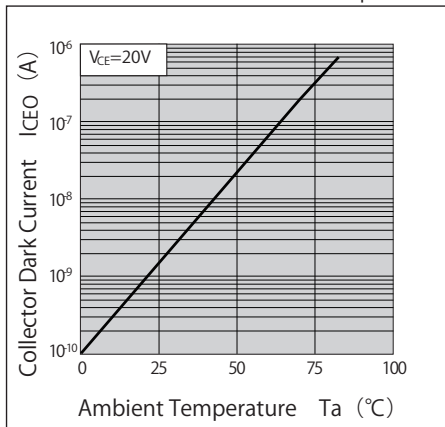
暗電流－周囲温度特性 (代表例) Collector Dark Current vs. Ambient Temperature
