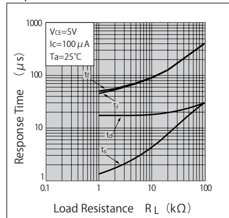
応答時間－負荷抵抗特性 (代表例) Response Time vs. Load Resistance
