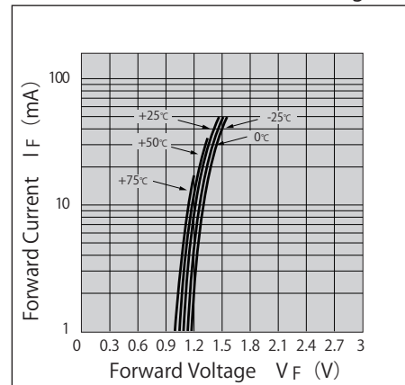
順電流－順電圧特性 (代表例) Forward Current vs. Forward Voltage
